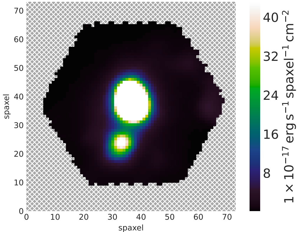
Emission line Gaussian flux: H-alpha 6564
