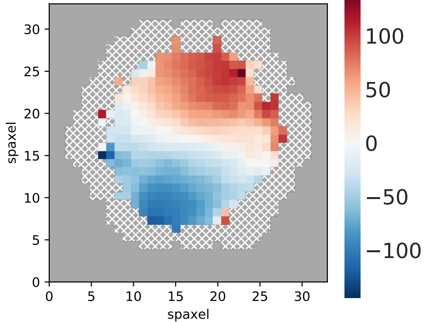
Emission line Gaussian velocity: H-alpha 6564
