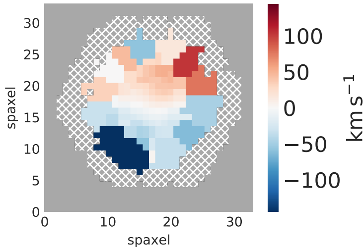
7443-12701 stellar_vel
