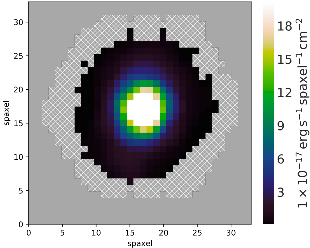
Emission line Gaussian flux: H-alpha 6564
