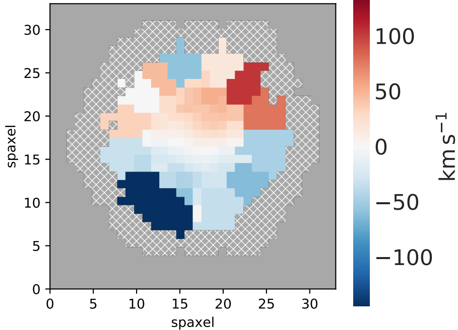
Stellar velocity
