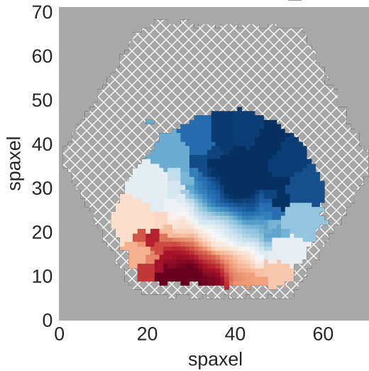
7443-12701 stellar_vel
