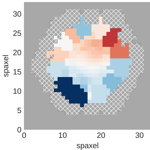
8485-1901 stellar_vel
