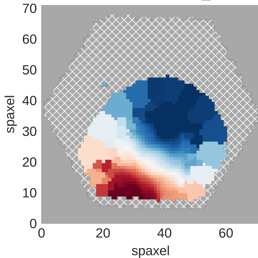
7443-12701 stellar_vel
